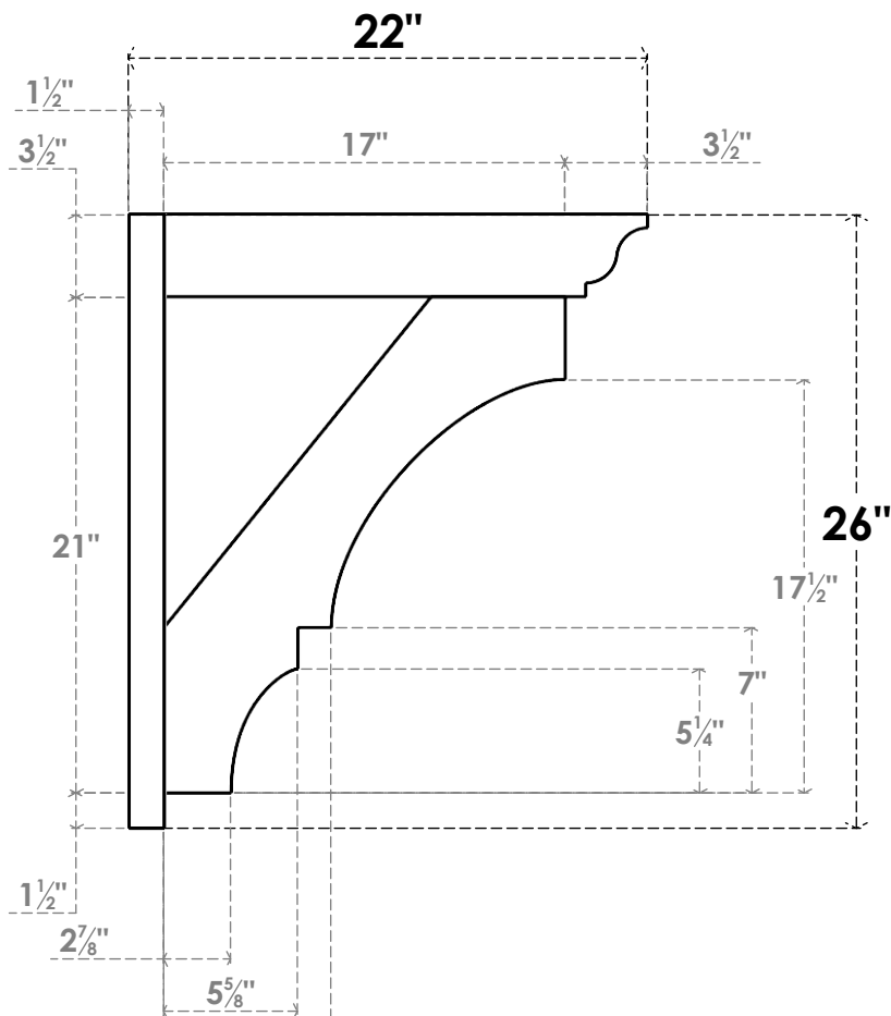
SIDE PROFILE
